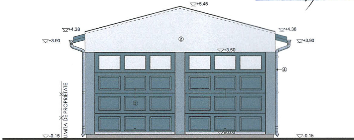
FATADA PRINCIPALA
